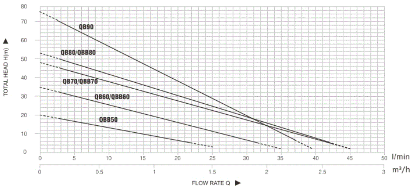
PERFORMANCE CHART AT n=2900rpm
